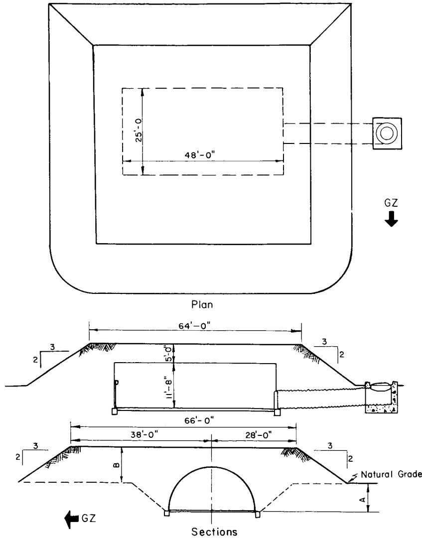
Fig. 8—Earth configuration, 25-ft-span structure. For structure 3.2a, A = 5.0 ft, B = 12 ft; for 3.2b, A = 3.0 ft, B = 14 ft; and for 3.2c, A = 1.5 ft, B = 15.5 ft.
